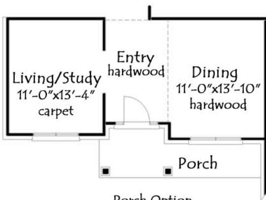
Porch Option required for Bedroom 6 option Elevation-B and C
